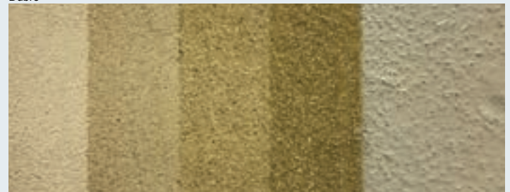
Concrete Primer Basecoat and Silica Sand Broadcast Coat 2nd Basecoat Silica Sand Broadcast Coat Pigmented Topcoat
